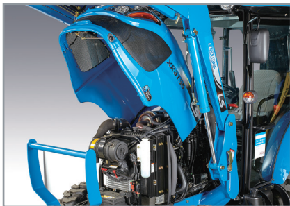
Easy open one-piece hood Provides accessibility for easy maintenance
